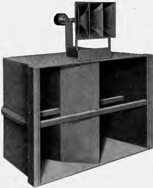
FIG. 4. Stage loud speaker equipment.
